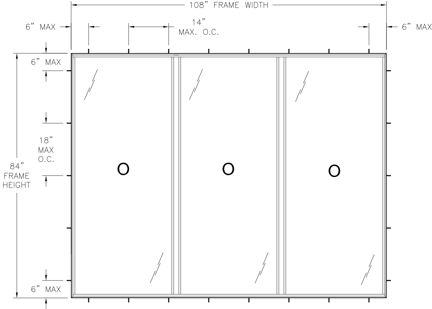
400/475 VINYL TRIPLE PICTURE WINDOW EXTERIOR VIEW FRAME INSTALLATION
