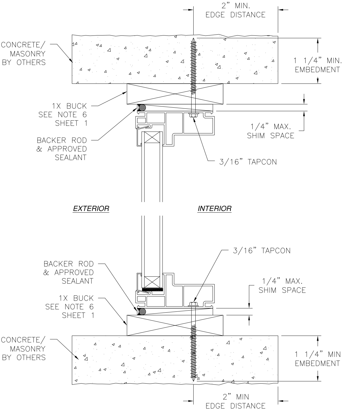
VERTICAL CROSS SECTION CONCRETE/MASONRY WITH 1X BUCK INSTALLATION FOR CONCRETE/MASONRY INSTALLATION WITHOUT 1X BUCK REFER TO JAMB INSTALLATION DETAILS
