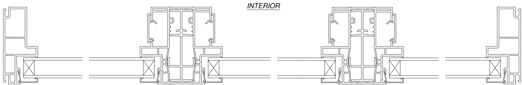
HORIZONTAL CROSS SECTION FINLESS FRAME
