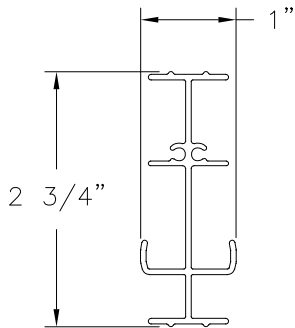
COMMON JAMB REINFORCEMENT (208A) ALUMINUM 6063-T5
