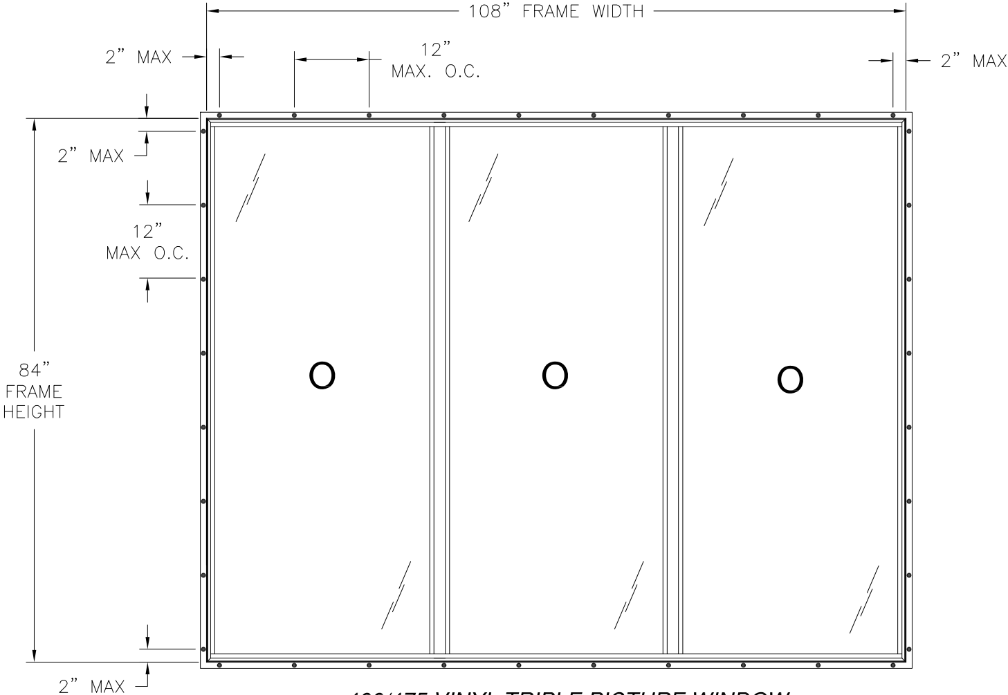
400/475 VINYL TRIPLE PICTURE WINDOW EXTERIOR VIEW FIN INSTALLATION
