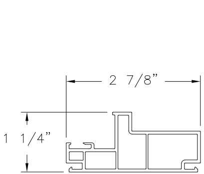
MAIN FRAME (BP4003) EXTRUDED RIGID PVC
