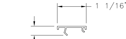
COMMON JAMB FILL COVER EXTRUDED RIGID PVC
