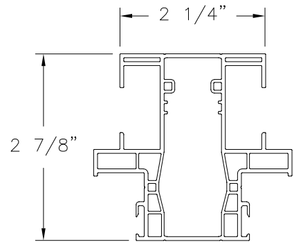
COMMON JAMB (BP4010) EXTRUDED RIGID PVC
