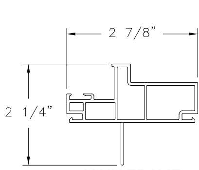
MAIN FRAME FIN INSTALLATION (BP4003) EXTRUDED RIGID PVC
